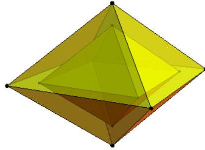
(b) Nested regular octahedra
